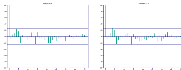
Figure 2. ACF and PACF of ASPI
